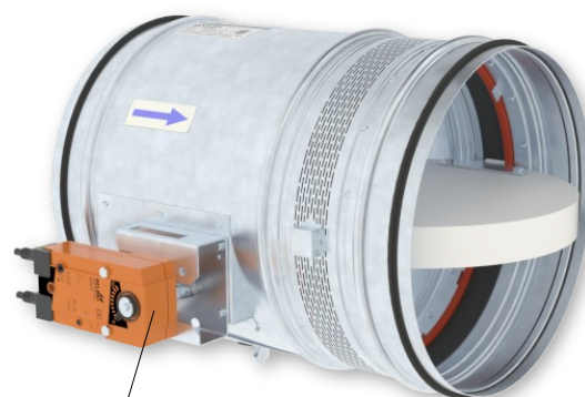
Servopohon
